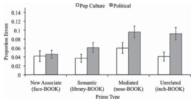
Figure 2. Error rates as a function of prime type and target type.
